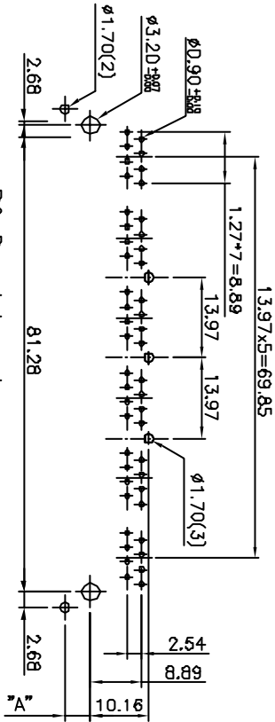
PC Board Layout Component Side Shown General Tolerance \pm 0.05
